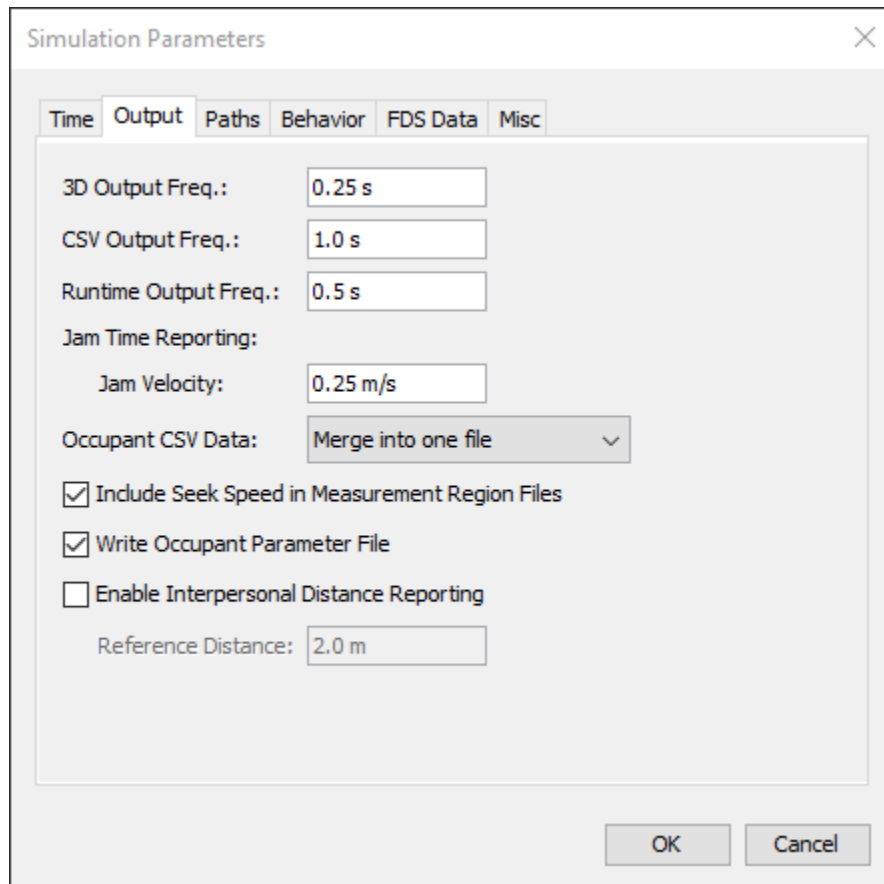
Figure 138. The Output tab of the Simulation Parameters dialog
