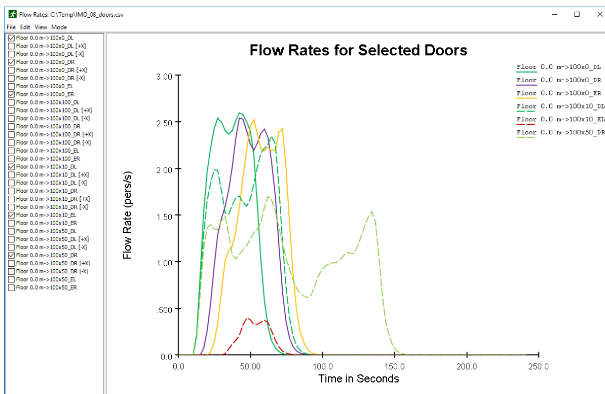
Figure 145. A time history plot for door flow rates
