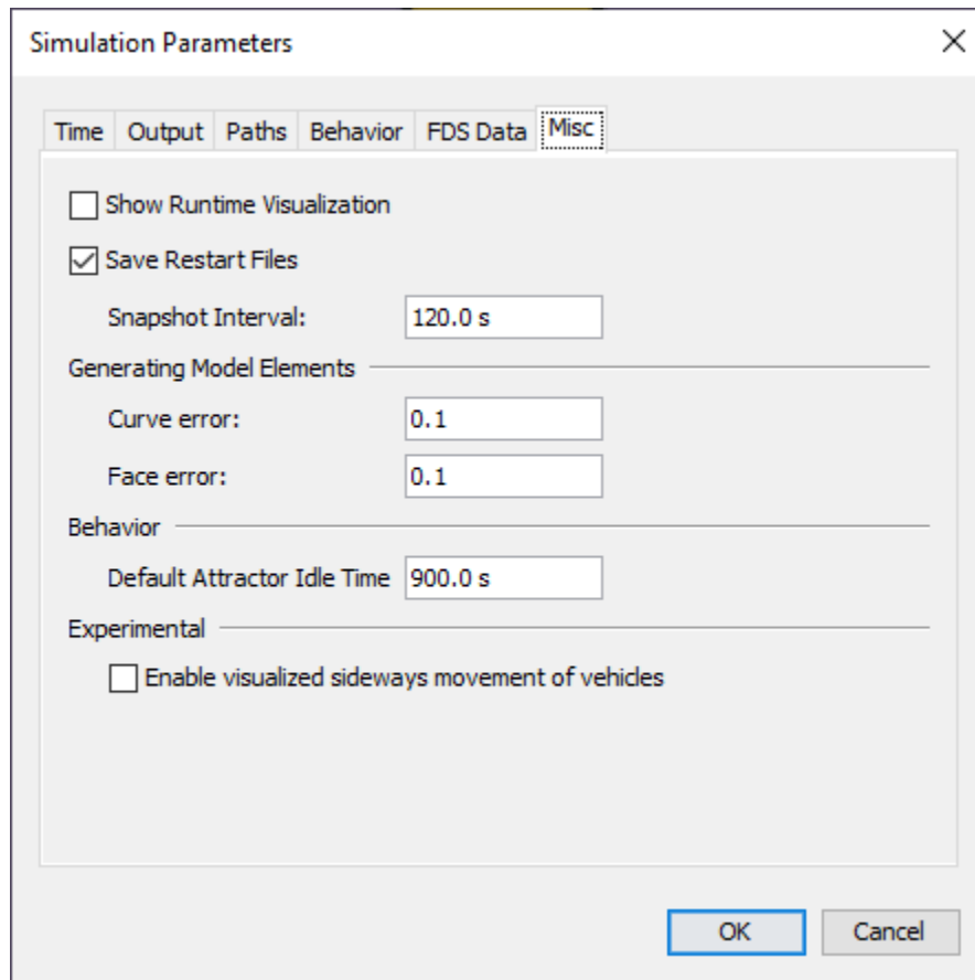
Figure 142. The Miscellaneous tab of the Simulation Parameters dialog
