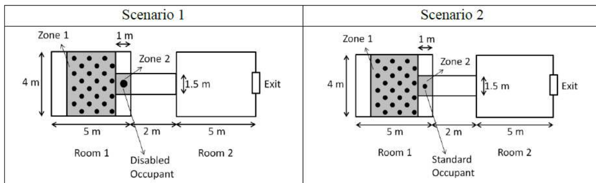
Figure 157. Geometry of movement disabilities verification (Verif.2.10). Figure from NIST Technical Note 1822, 2013.
