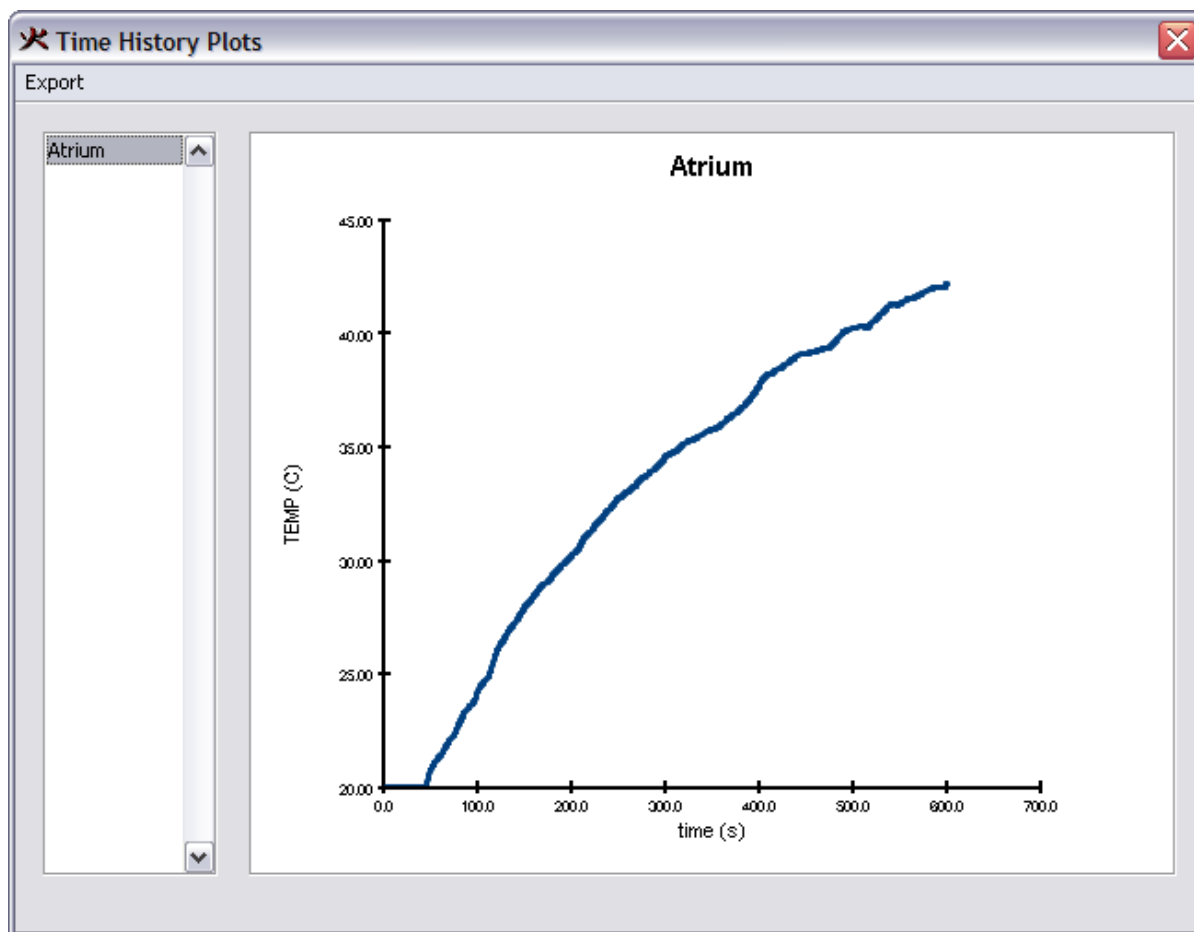
Figure 149. Time History Results
