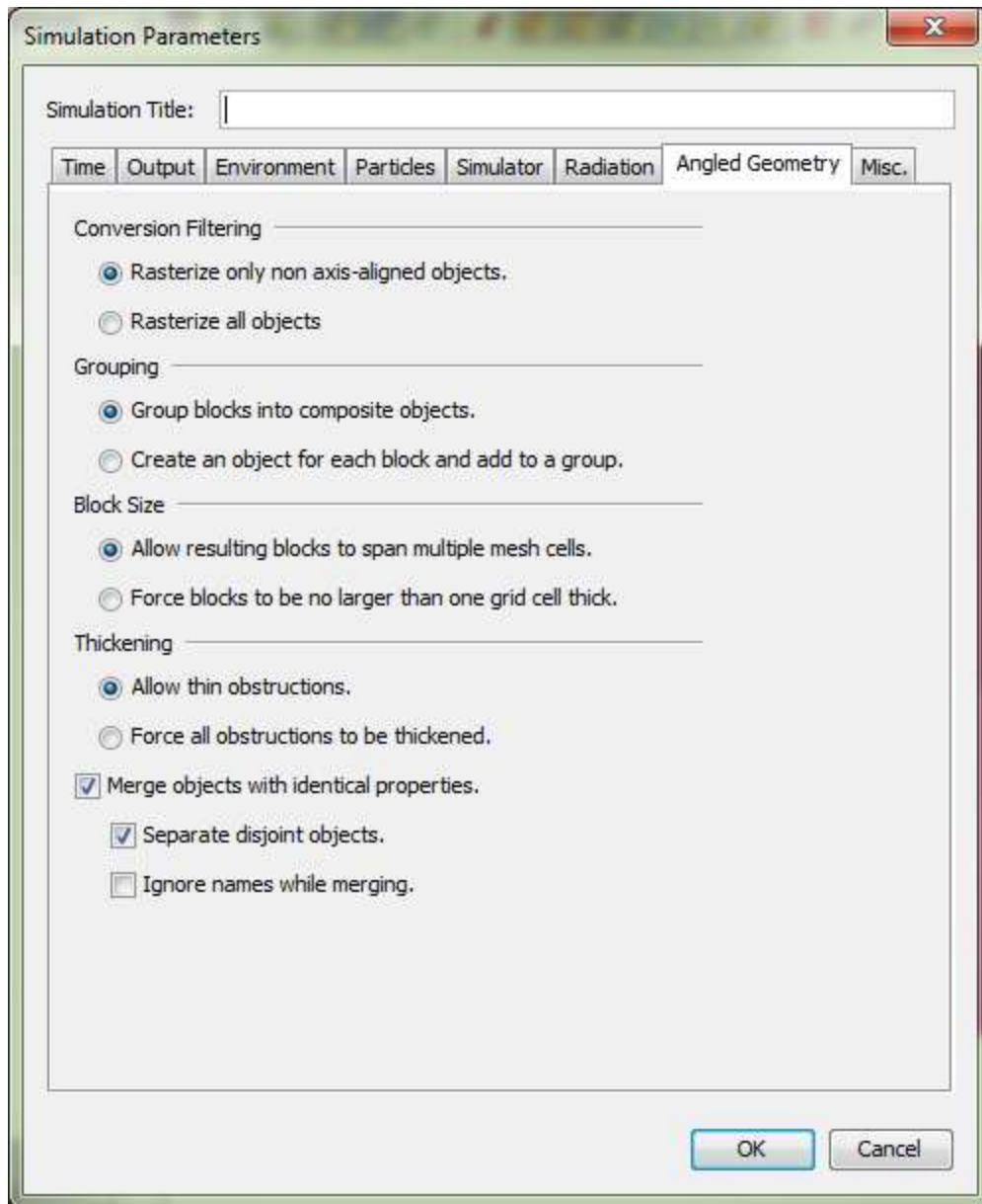
Figure 136. Angled Geometry tab of the simulation parameters dialog
