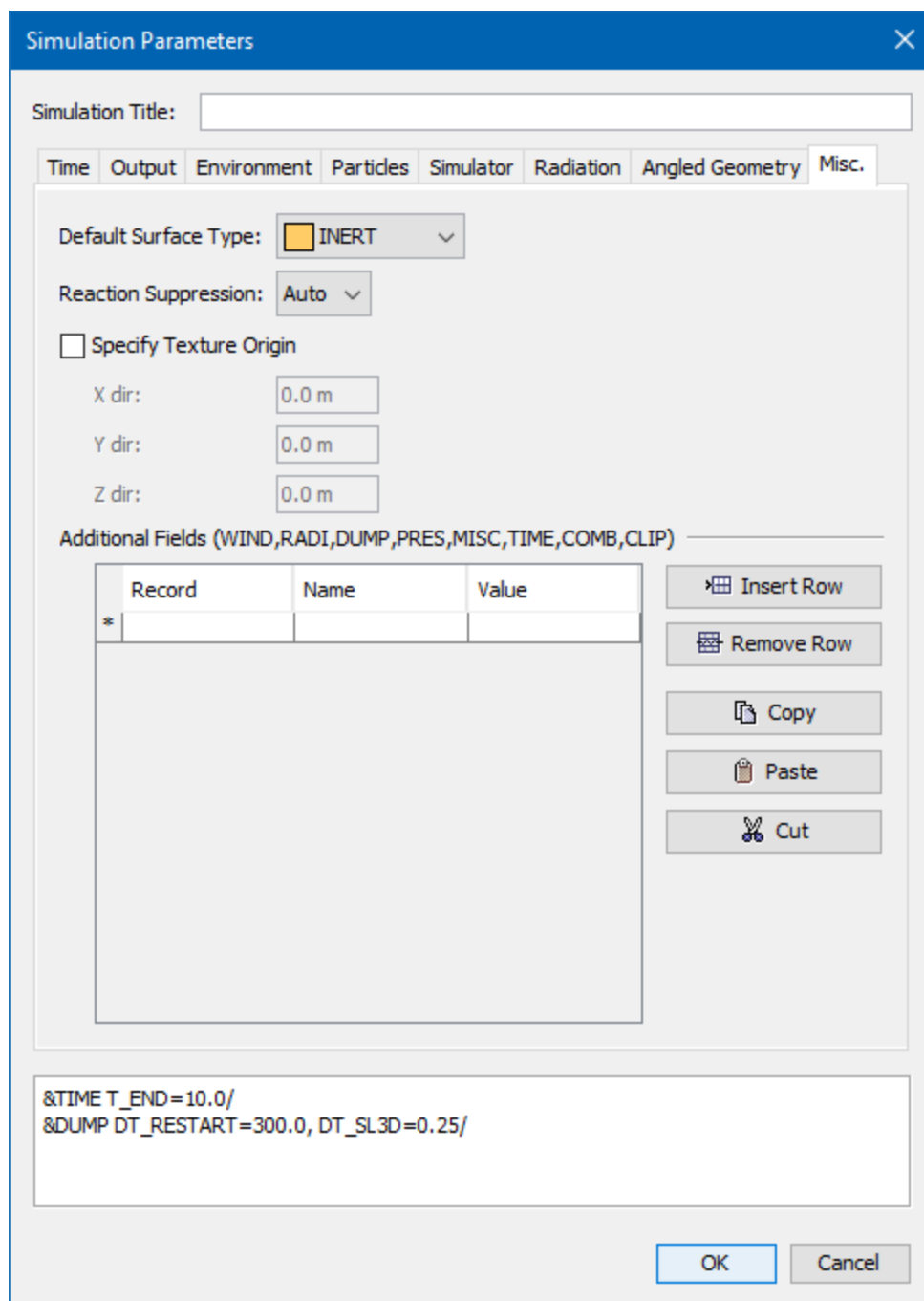
Figure 142. Misc. tab on the Simulation Parameters dialog
