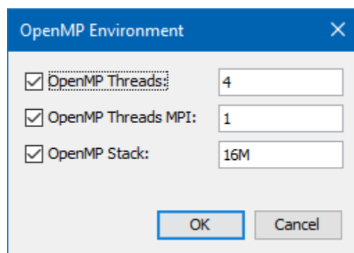
Figure 143. The OpenMP Environment dialog
