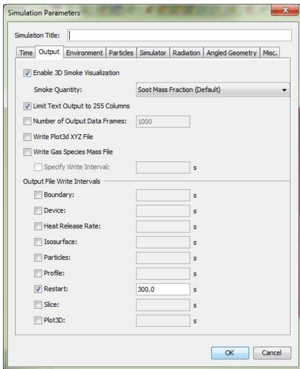
Figure 131. Output tab of the simulation parameters dialog
