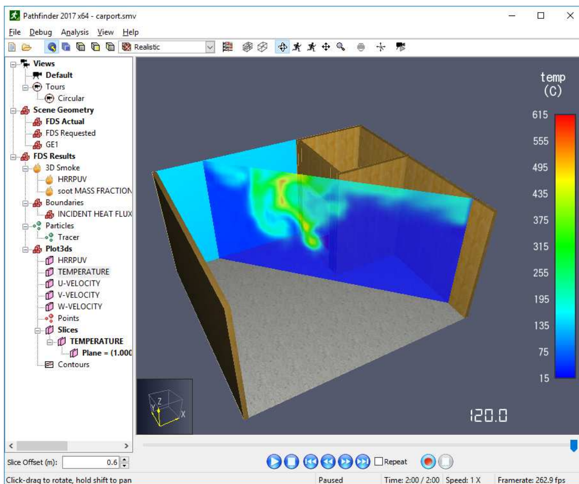
Figure 128. An angled temperature slice through Plot3D data shown in the 3D Results
