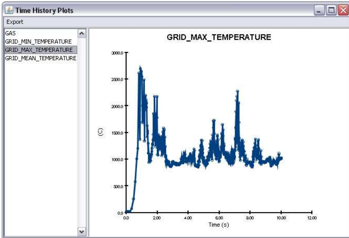
Figure 129. An example of statistic output
