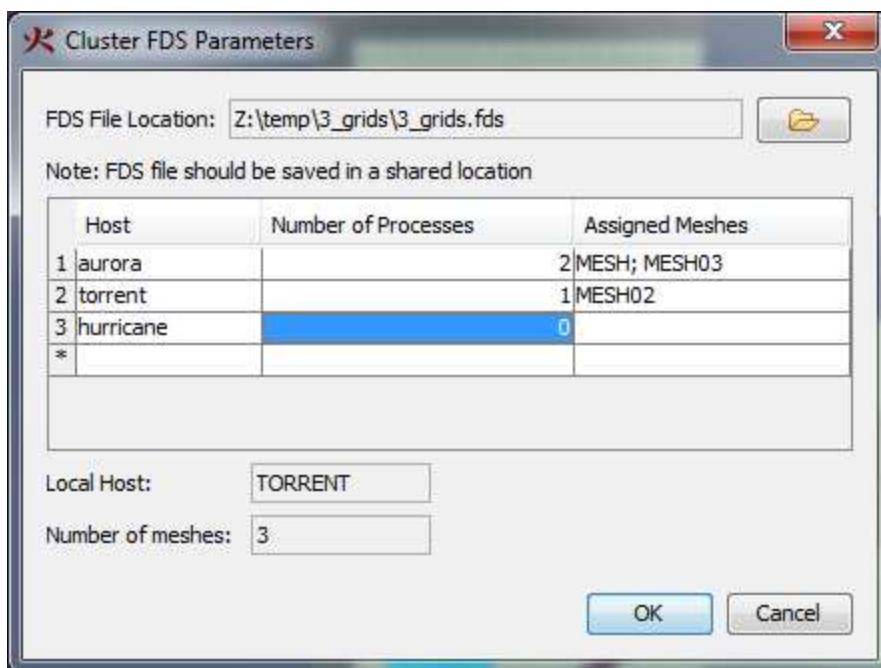
Figure 146. The Cluster FDS Parameters dialog
