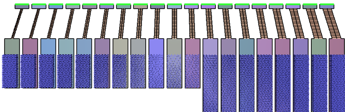
Figure 34: Pathfinder model used to study stair flow rates. The door widths range from 0.7 to 3.0 m. Entry corridor width is 5 m. Stairs have a total rise of 7 m and a run of 11 m.
