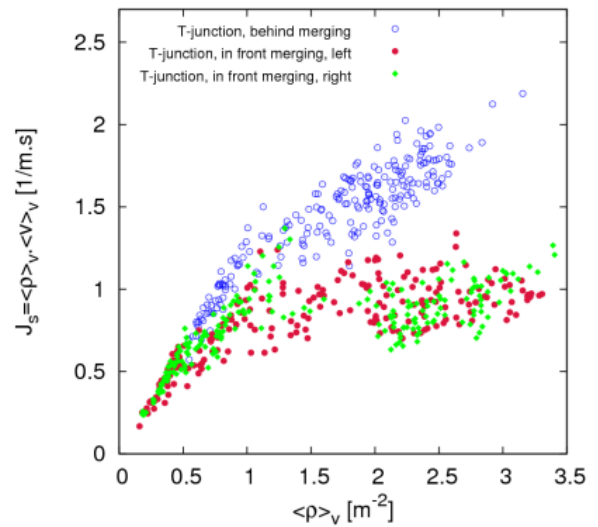
Figure 18: Fundamental diagrams for T-junction (Ref. Zhang et al., 2012).
